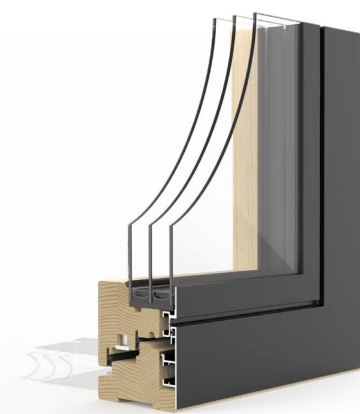
KOMFORT ULTIMO U_g = 0,50 \text{ W/m}^2\text{K} U_w = 0,74 \text{ W/m}^2\text{K}
