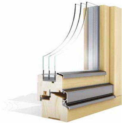
NATURA OPTIMO U_g = 0,50 \text{ W/m}^2\text{K} U_w = 0,74 \text{ W/m}^2\text{K}
